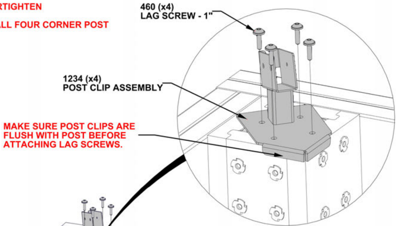
A4M01234 POST CLIP ASSEMBLY (x4)
